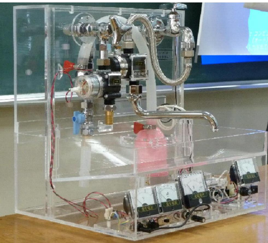
hydro power plant
