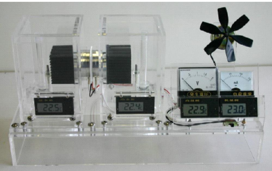
Ocean thermal power generation system
