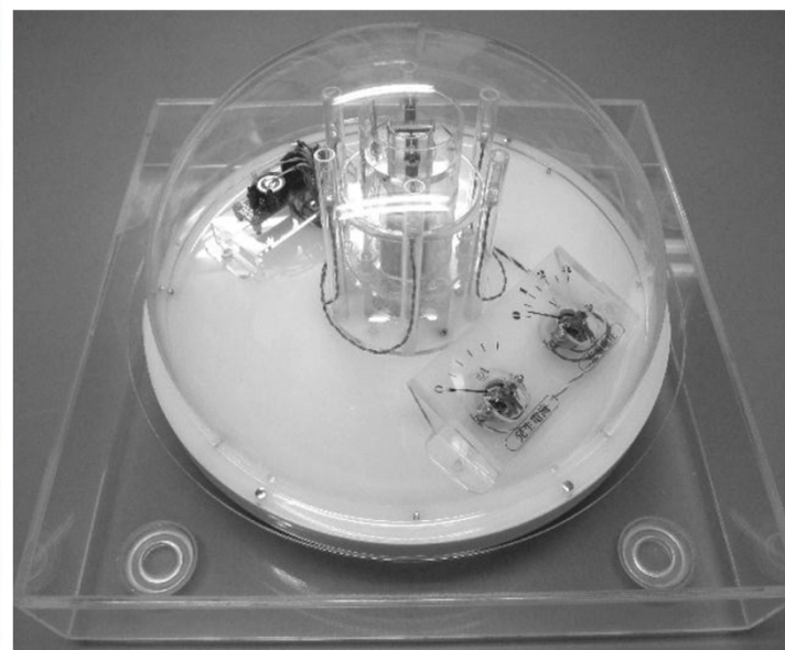
Wave power generation system
